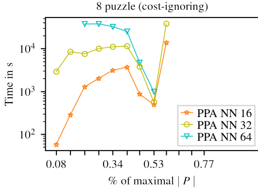
Figure 1: Excerpt of results by Vea22 for their best-performing PPA variant, on one of their benchmarks (8-puzzle cost-ignoring), for different hidden-layer sizes.
